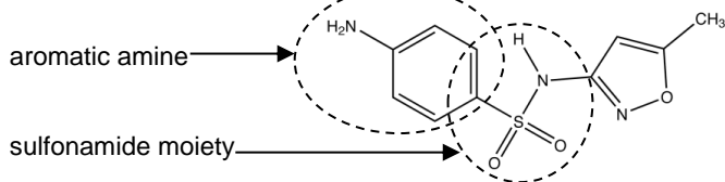
Figure: sulfamethoxazole
